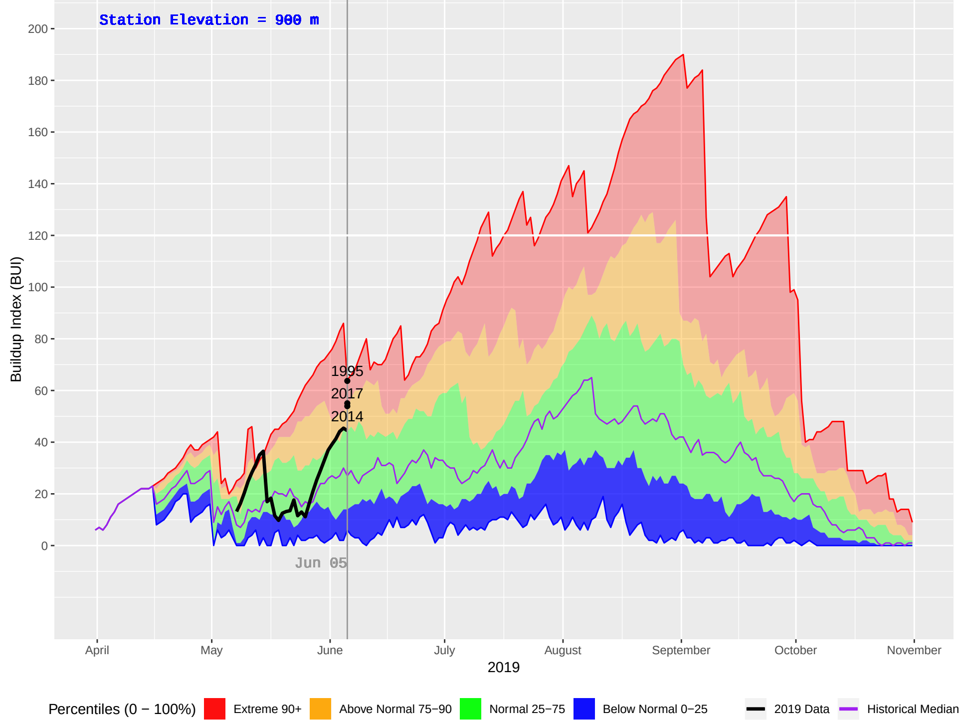
UPPER FULTON (169) : Historical (1986–2018), Current (2019) Daily Buildup Index (BUI)
