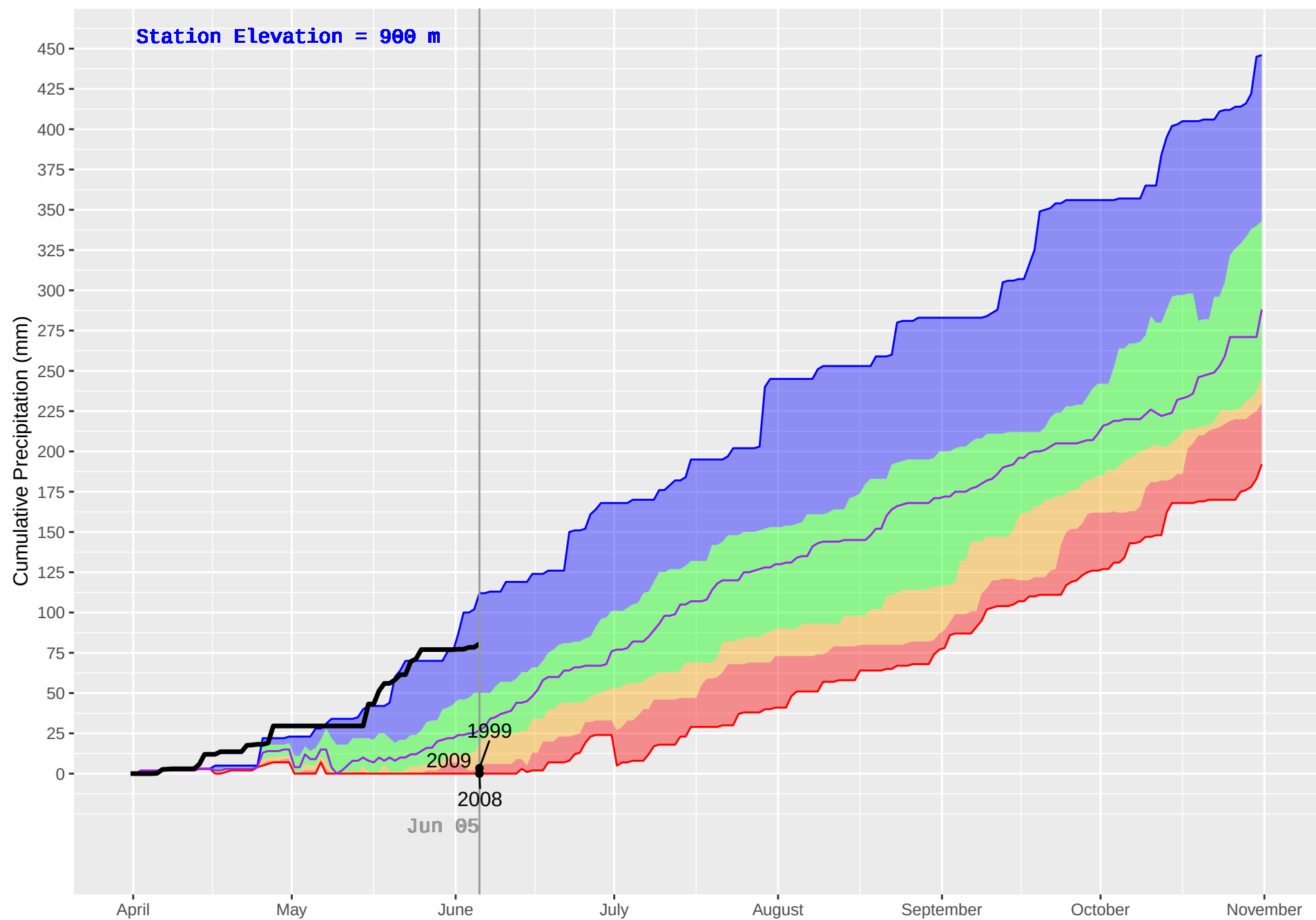
UPPER FULTON (169) : Historical (1986–2018), Current (2019) Daily Cumulative Precipitation
