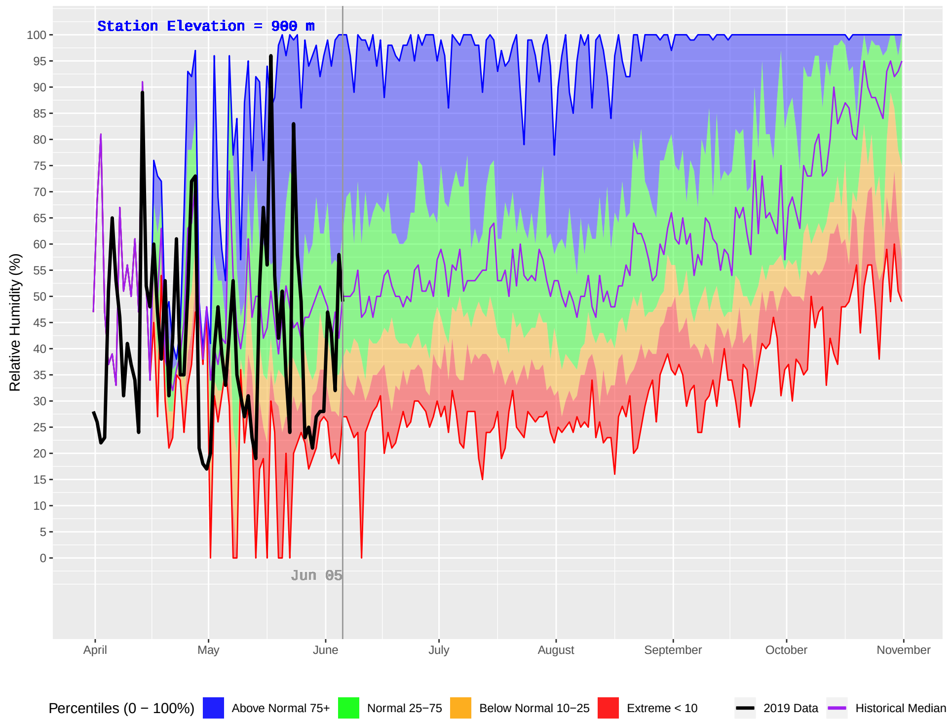
UPPER FULTON (169) : Historical (1986–2018) and Current (2019) Daily Relative Humidity
