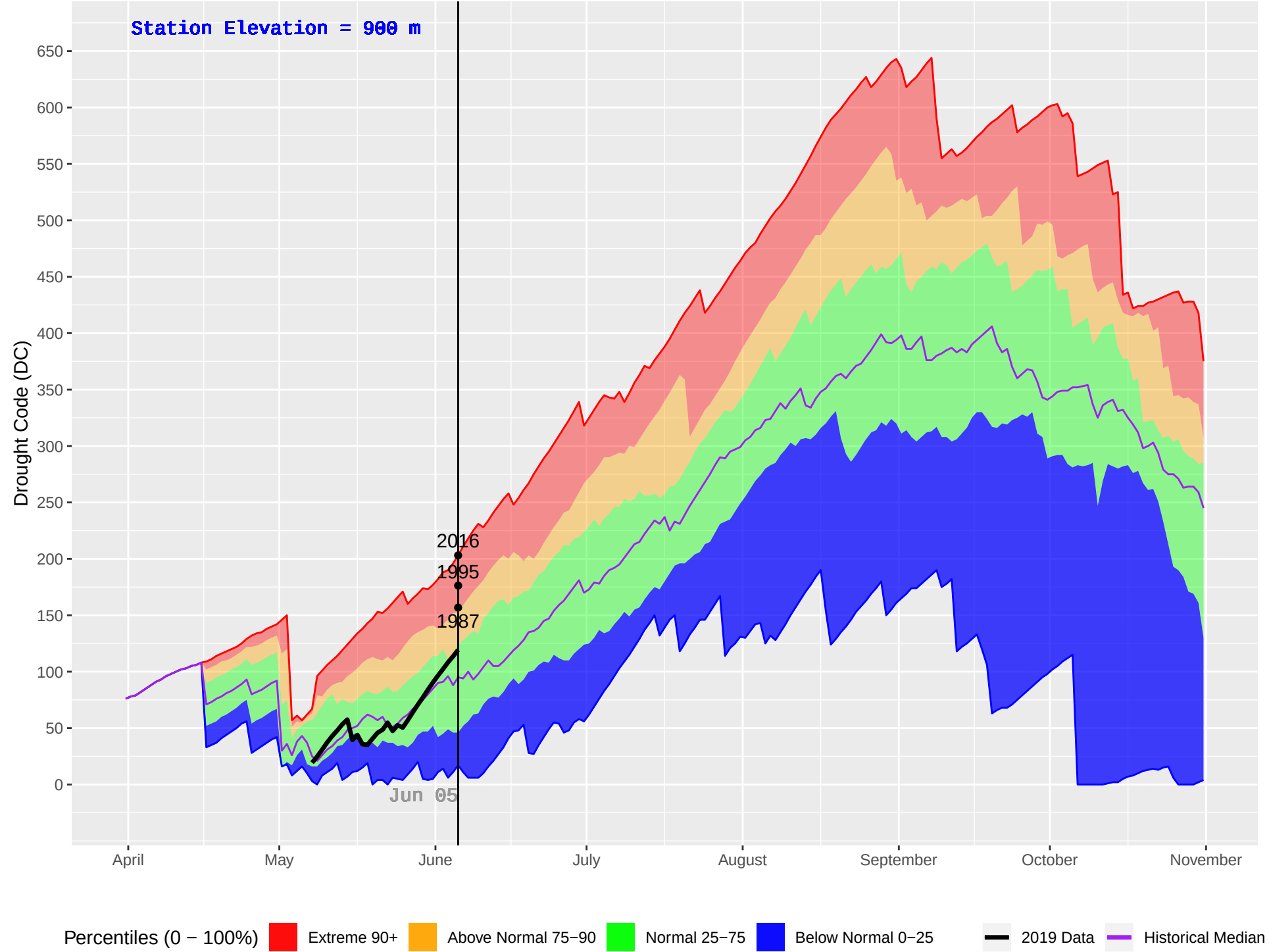
UPPER FULTON (169) : Historical (1986–2018) and Current (2019) Daily Drought Code (DC)
