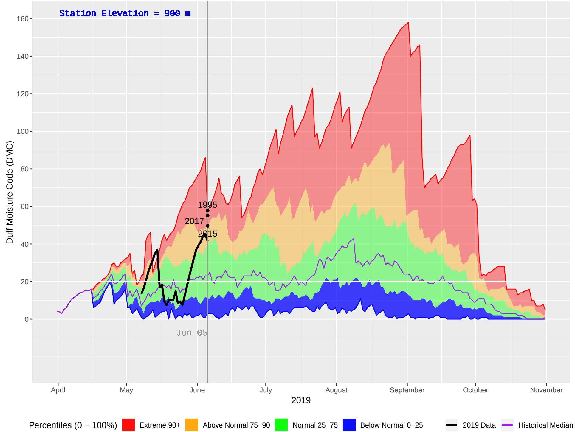
UPPER FULTON (169) : Historical (1986–2018), Current (2019) Daily Duff Moisture Code (DMC)
