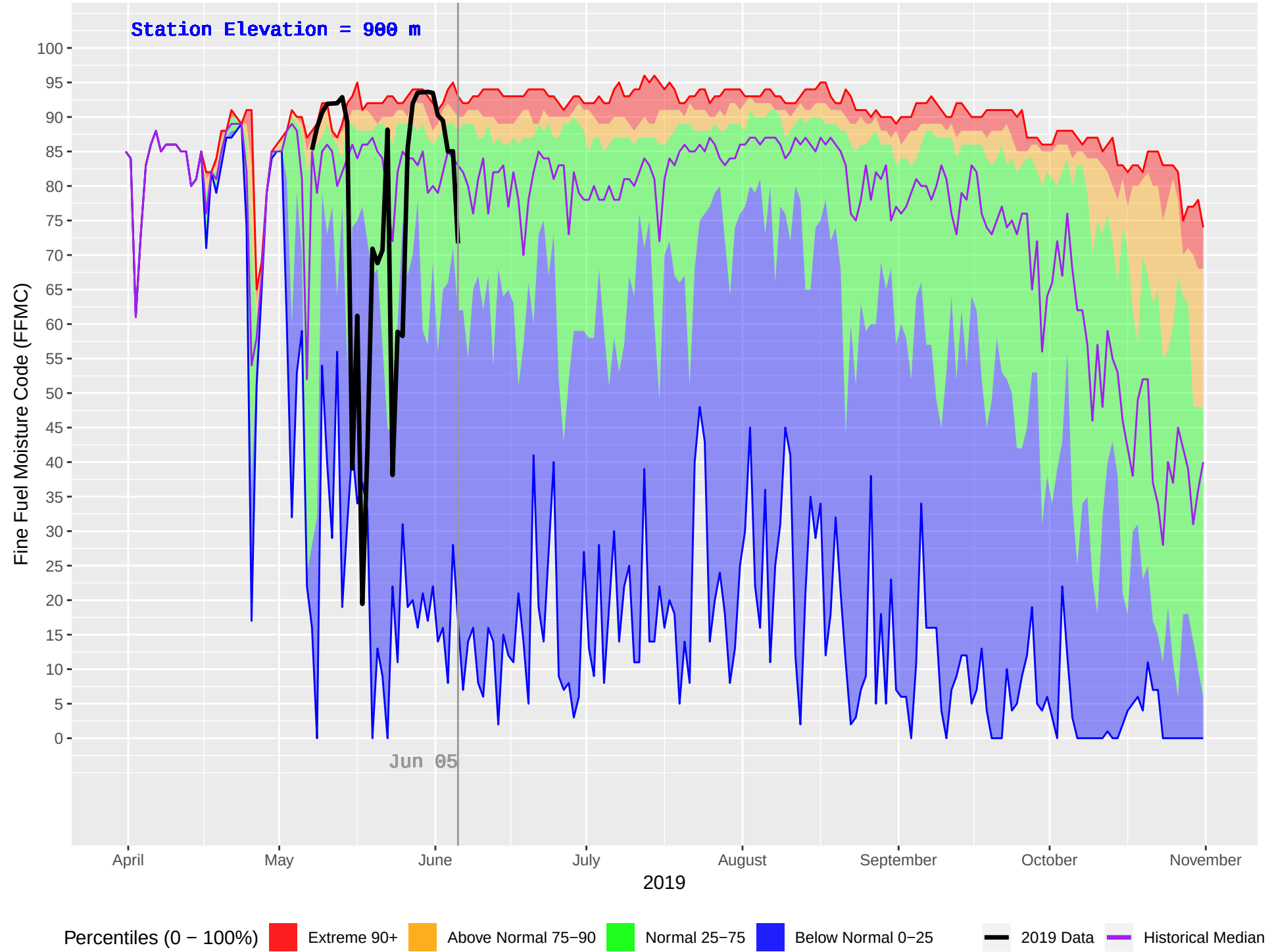
UPPER FULTON (169) : Historical (1986–2018) and Current (2019) Daily Fine Fuel Moisture Code (FFMC)
